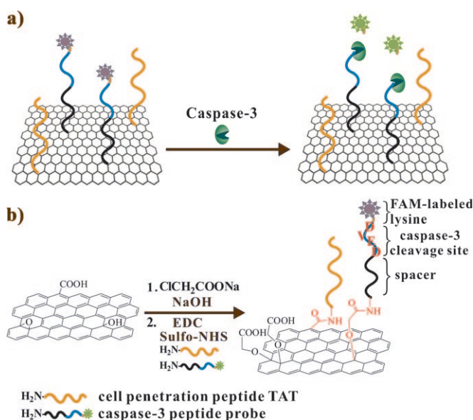
Scheme 1. a) Caspase-3 detection using GO–peptide conjugate.
